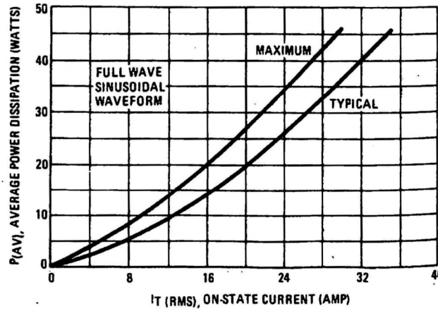
FIGURE 2 – POWER DISSIPATION
