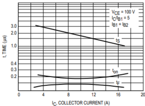
Figure 5. Resistive Switching Performance
