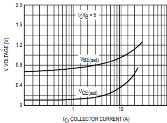
Figure 3. "On" Voltages
