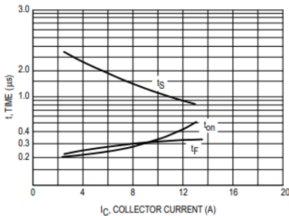
Figure 5. Switching Times versus Collector Current
