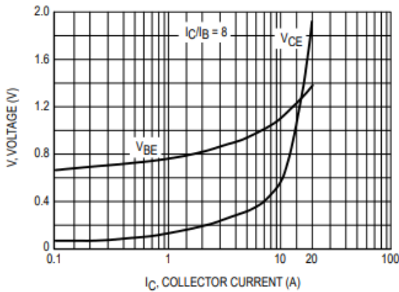
Figure 3. "On" Voltages
